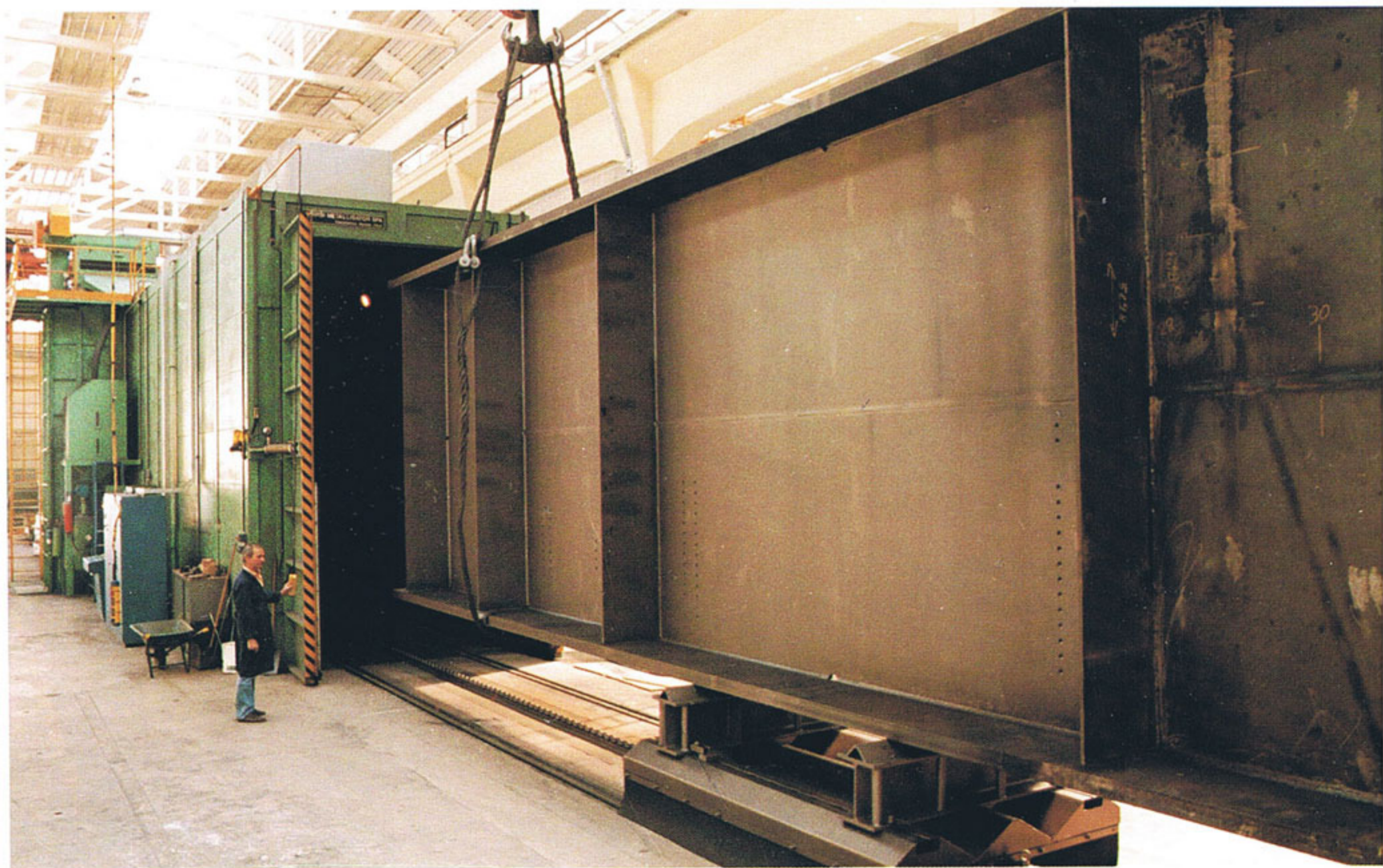
IMPIANTI PER LA GRANIGLIATURA AUTOMATICA DI GRANDI COMPONENTI E STRUTTURE AUTOMATIC SHOTBLAST EQUIPMENT FOR LARGE STEEL CONSTRUCTIONS INSTALLATIONS POUR LE GRENAILLAGE AUTOMATIQUE DES GRANDES COMPOSANTS ET STRUCTURES
