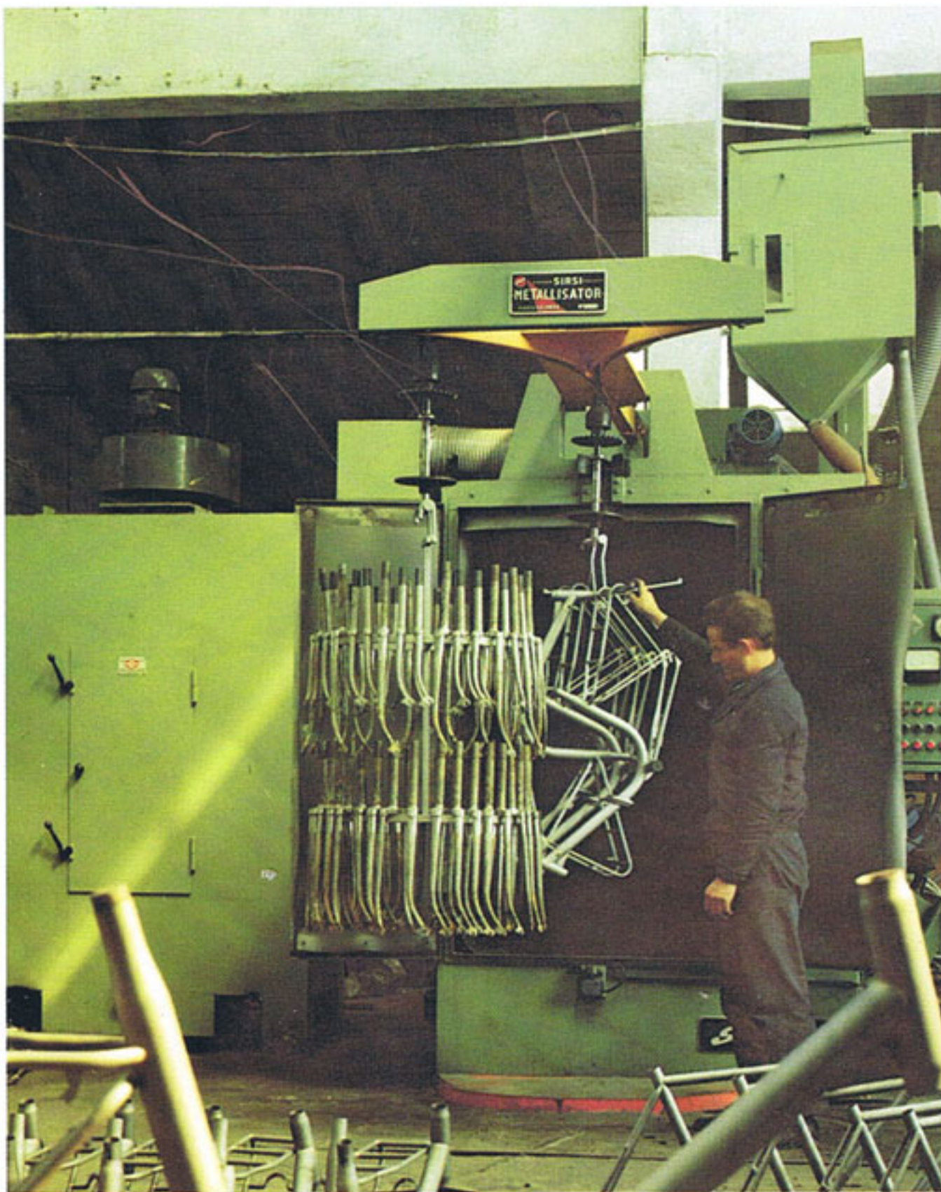
GRANIGLIATRICI A GANCI. PORTATA 500 ÷ 1000 KG HANGERS SHOTBLAST UNITS. CAPACITY 500 ÷ 1000 KGS GRENAILLEUSES A CROCHETS. CAPACITE 500 ÷ 1000 KGS
