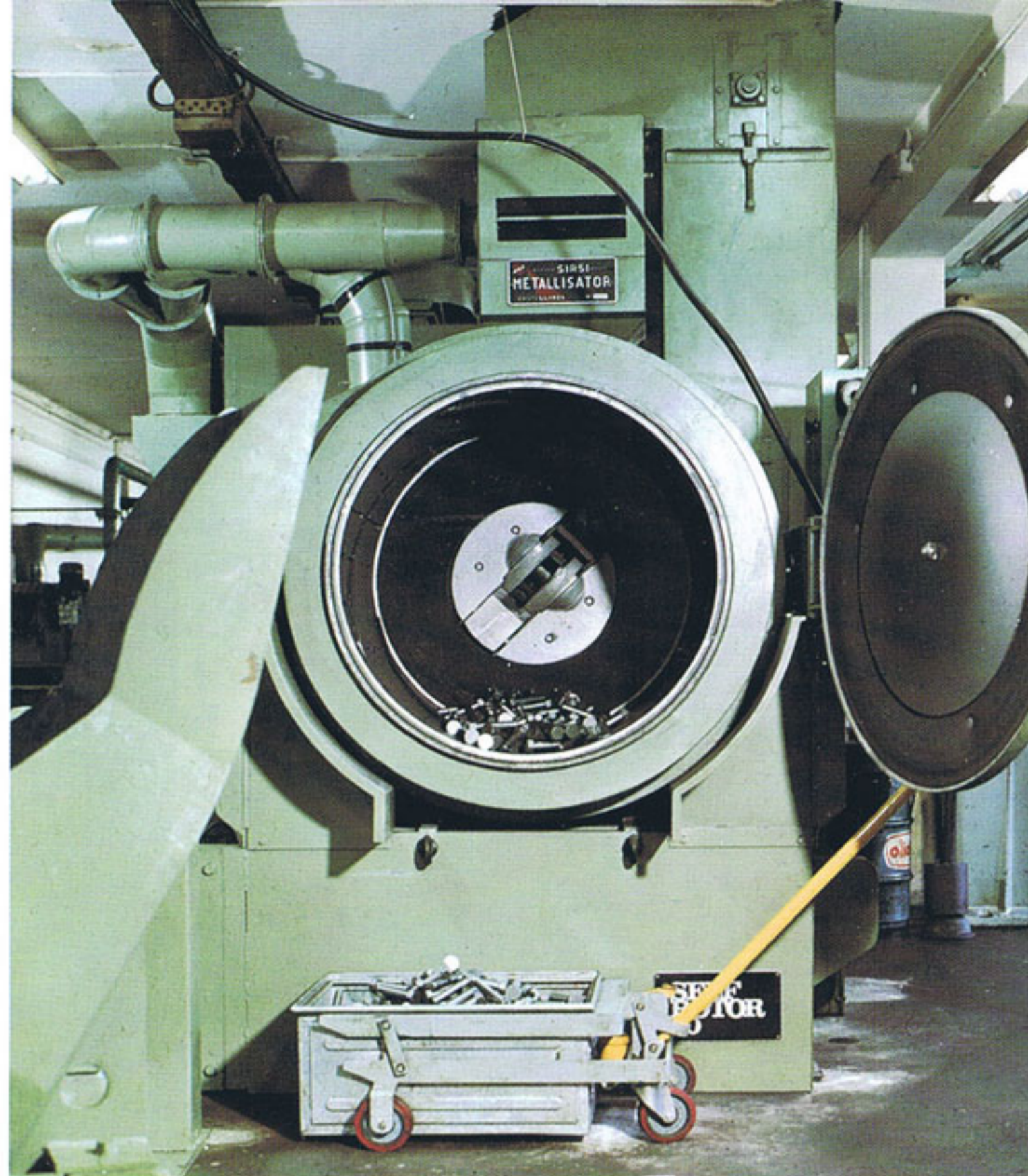
GRANIGLIATRICI A TAMBURO. PORTATA 80 ÷ 1500 KG DRUM SHOTBLAST UNITS. CAPACITY 80 ÷ 1500 KGS GRENAILLEUSES A TAMBOUR. CAPACITE 80 ÷ 1500 KGS
