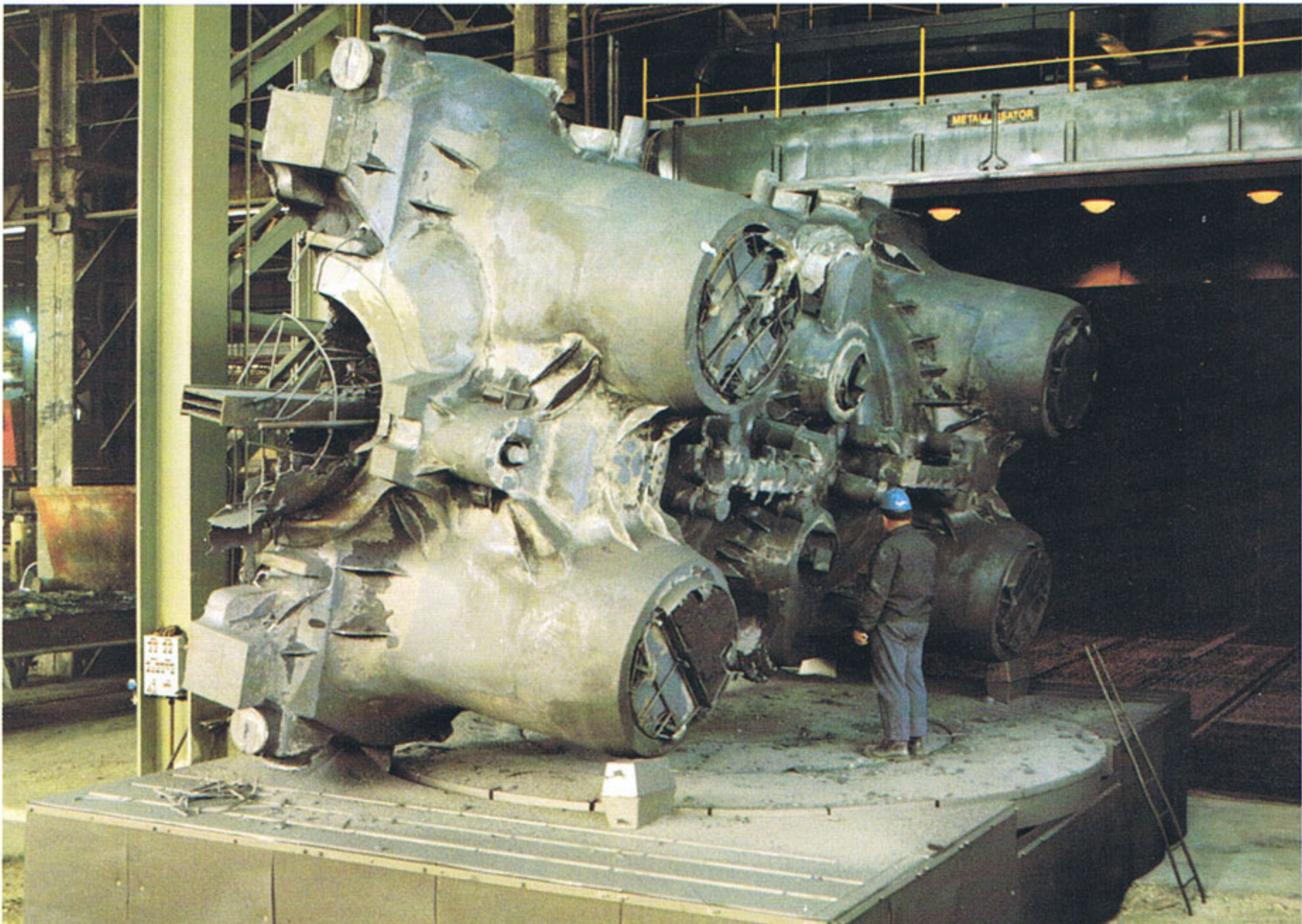
IMPIANTI DI STERROGRANIGLIATURA A CARRO MOBILE. PORTATA 40 ÷ 150 TON DESANDING SHOTBLAST EQUIPMENT WITH MOBILE BOGIE. CAPACITY 40 ÷ 150 TONS
